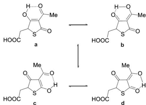
Scheme 2. Enol-enol equilibrium of the 3-acetyl-5-carboxymethylthiotetronic acid ( 11 ).
