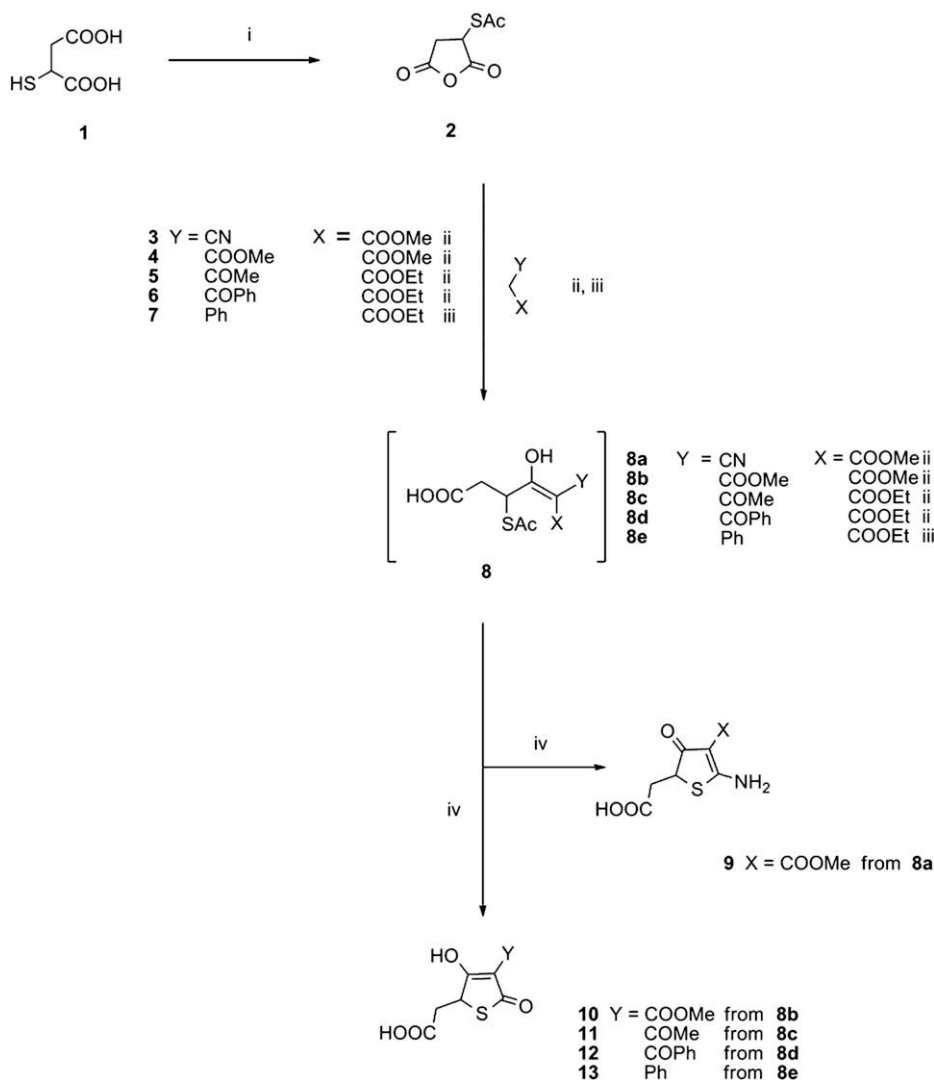
Scheme 1. Reagents and conditions: (i) \text{CH}_3\text{COCl} , reflux; (ii) NaH, THF; (iii) LDA, THF -78^\circ\text{C} ; (iv) MeOH, 2 M NaOH.
