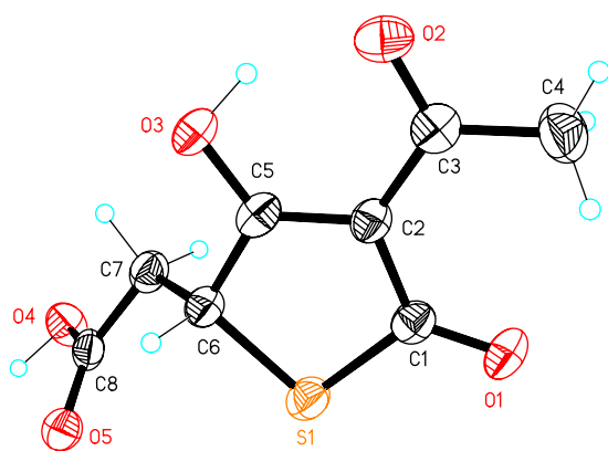
Figure 4. Molecular structure of 11 , the dashed line represents a hydrogen bond. Thermal ellipsoids drawn at the 50% probability level.
