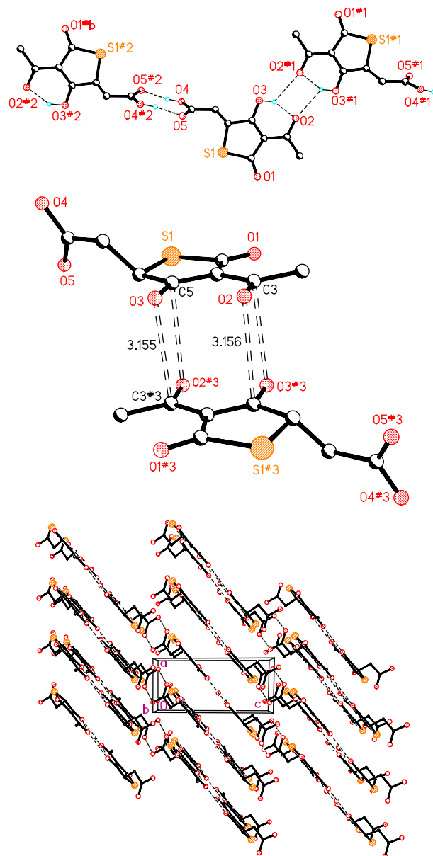
Figure 4. Molecular structure of 11 , the dashed line represents a hydrogen bond. Thermal ellipsoids drawn at the 50% probability level.
