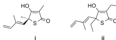
Figure 2. Thiolactomycin (i) and thiotetramycin (ii).
