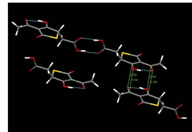
Figure 5. Intermolecular interactions in 11 : hydrogen-bonded chain with dashed lines representing hydrogen bonds (top) and \pi -stacking interactions (bottom). Symmetry transformations used to generate equivalent atoms: #1 -x-1, -y, -z+1 ; #2 -x+1, -y-1, -z ; #3 -x, -y, -z+1 .
